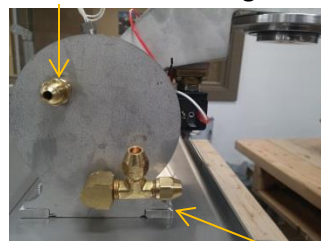
1.5700 Inlet fitting
